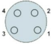
Socket, 4-pos.
